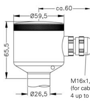
Field housing (IP 67)
