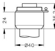
M12x1 4-pin (IP 67)
