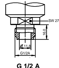
G 1/2 A
