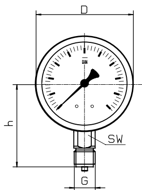
Connection bottom
