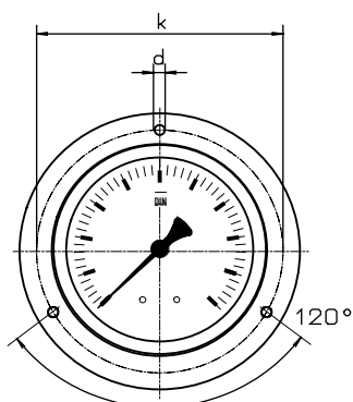
Front ange
