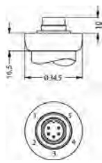
Binder Series 723 5-pin (IP 67)
