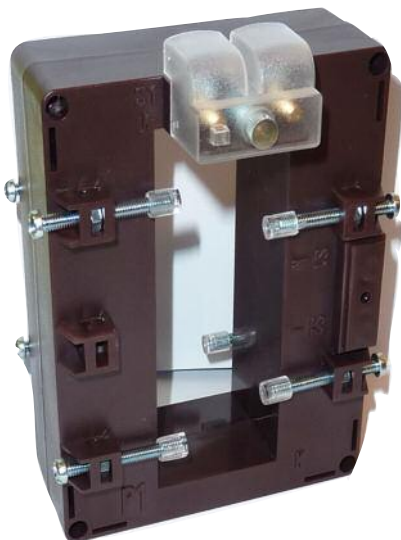
Plombierbare Klemmenabdeckung Sealable terminal cover (Option Option)
